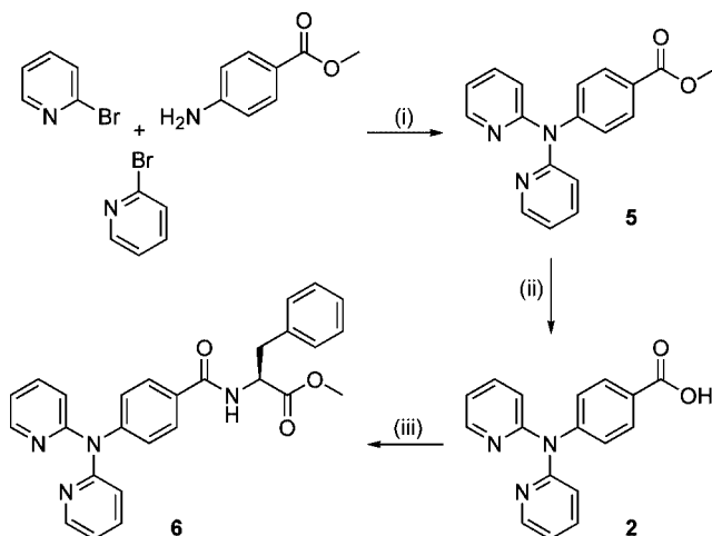
Scheme 2. Synthesis of the aromatic side chain dpa derivatives 2 , 5 and 6 : (i) K 2 CO 3 , KI (cat.), Cu(SO 4 ) 2 ·5H 2 O (cat.), phen (cat.), neat/7 h, 200 °C (52%); (ii) 1 M NaOH/16 h, room temp. (89%); (iii) HBTU, HOBT, H-Phe-OMe·HCl, DIPEA/20 h, 0 °C → room temp. (56%).
