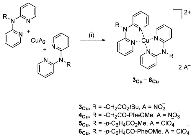
Scheme 3. Synthesis of the [\text{Cu}(\text{dpa})_2] complexes 3 Cu – 6 Cu : (i) MeOH, \Delta (50–75%).
