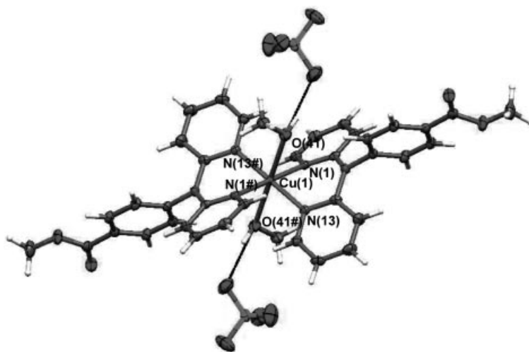
Figure 5. X-ray single crystal structure of 5 Cu (thermal ellipsoids at 50% probability).
