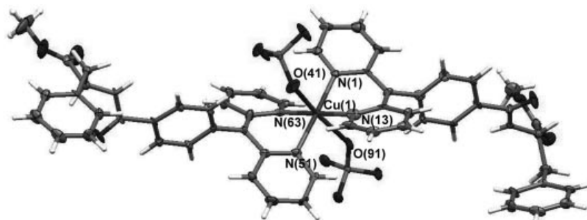
Figure 6. X-ray single crystal structure of 6 Cu (thermal ellipsoids at 50% probability).
