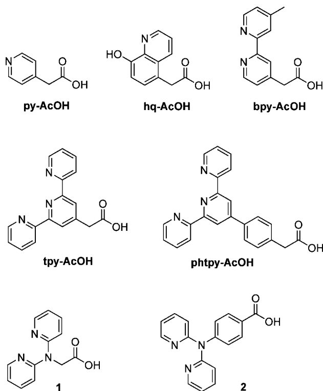
Figure 1. The heterocyclic acetic acid derivatives previously used for the synthesis of aeg-oligoligandosides [5b,14] and the dpa derivatives 1 and 2 prepared in this study.
