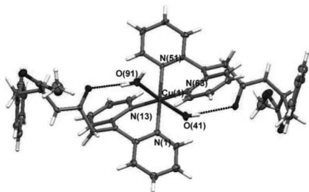
Figure 4. X-ray single crystal structure of 4 Cu dication (thermal ellipsoids at 30% probability). The nitrate counterions and methanol solvent molecules are omitted for clarity.
