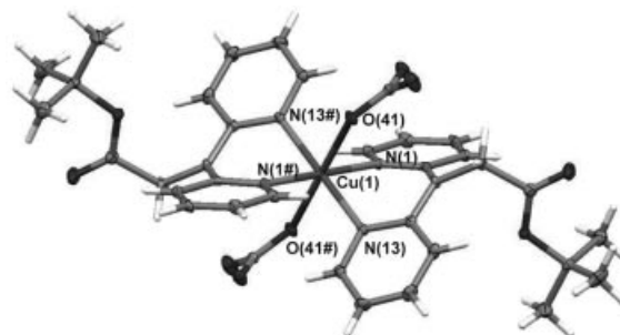
Figure 3. X-ray single crystal structure of 3 Cu (thermal ellipsoids at 50% probability).
